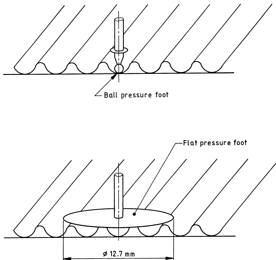
Figure 2 — Alternative pressure foot types for micrometer
