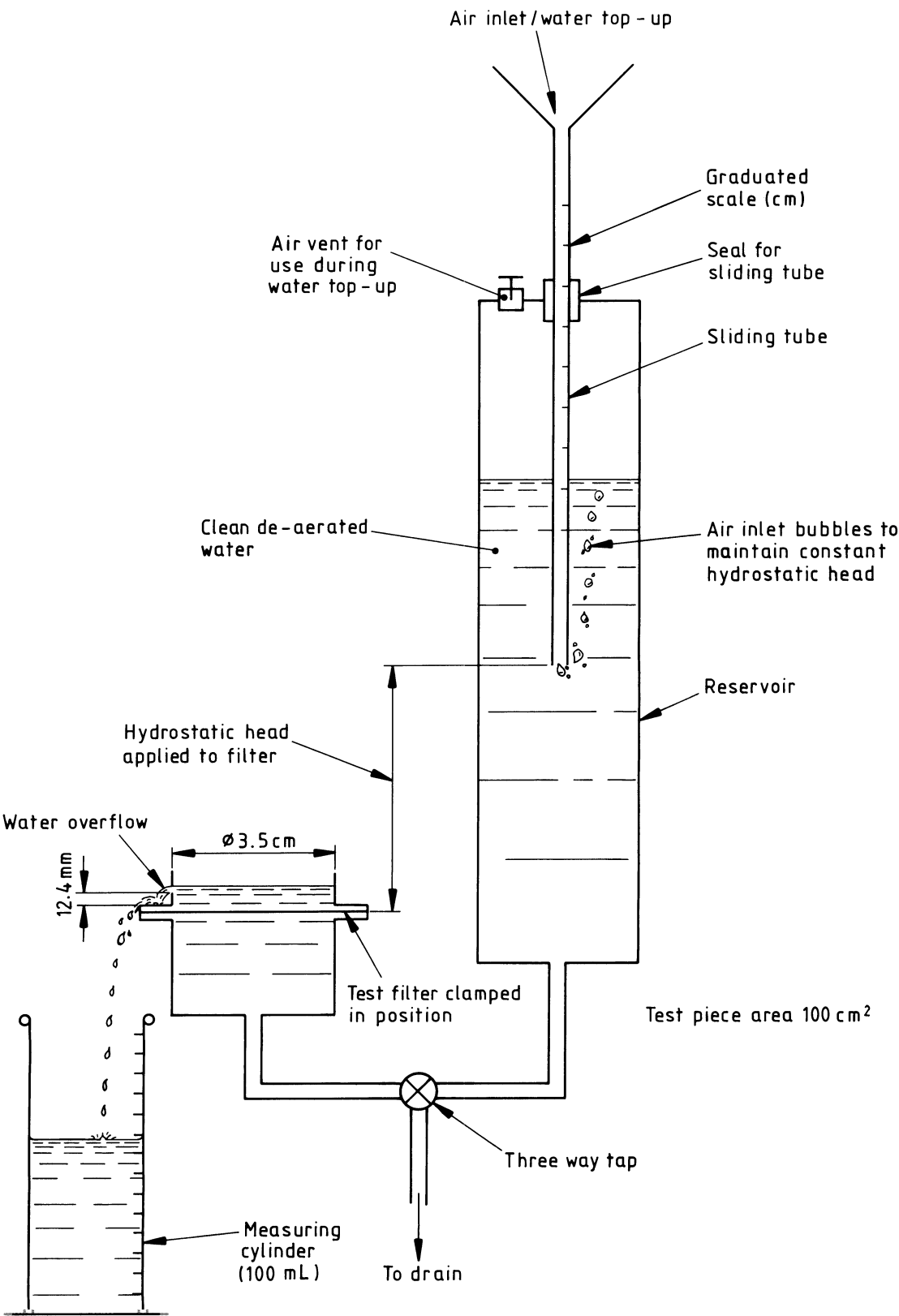
Figure 11 — Water filtration time apparatus (Herzberg)
