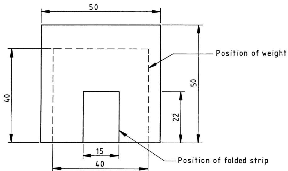
Figure 5 — Template for positioning the weight on the folded strip
