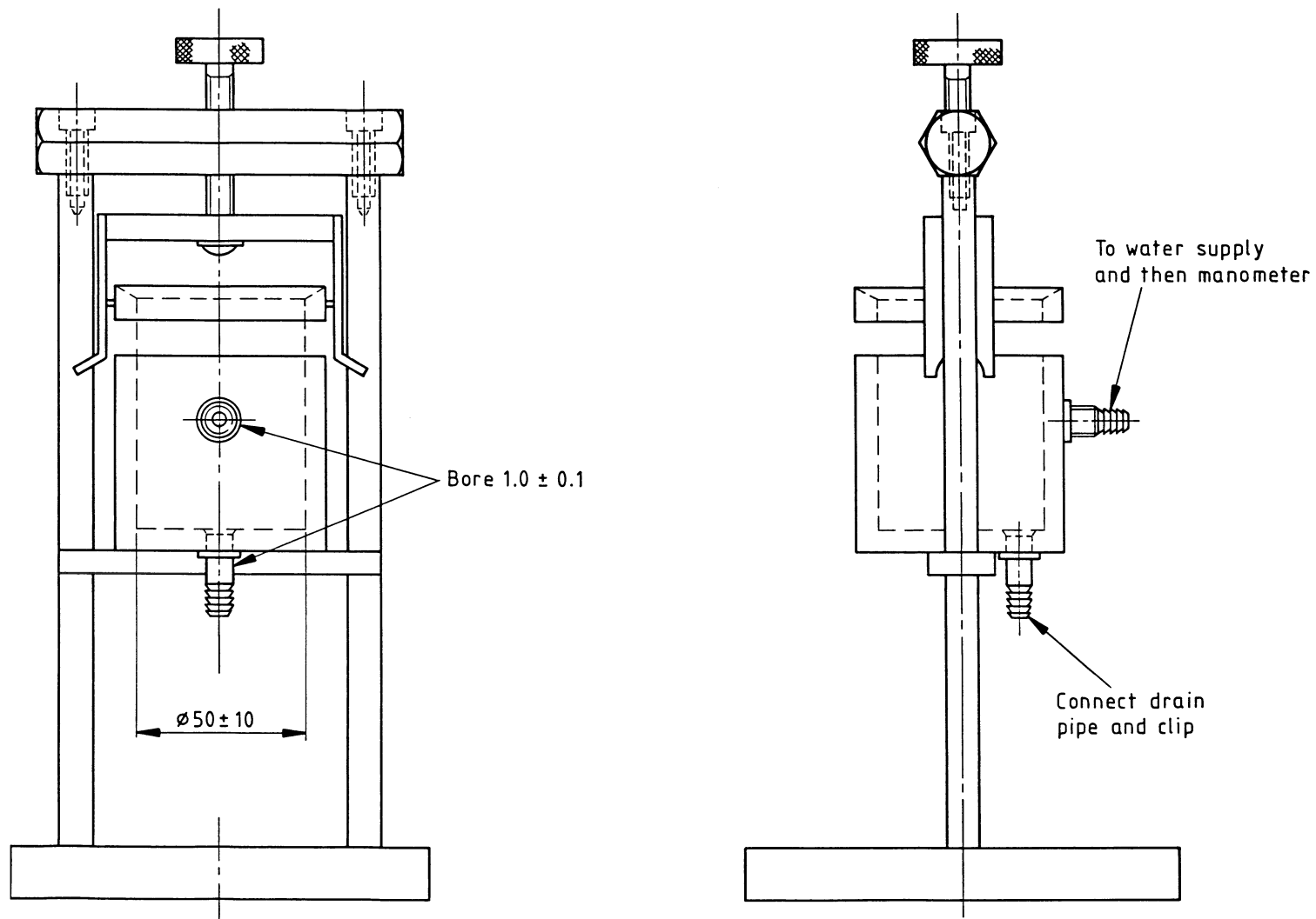
Figure 10 — Water resistance apparatus
